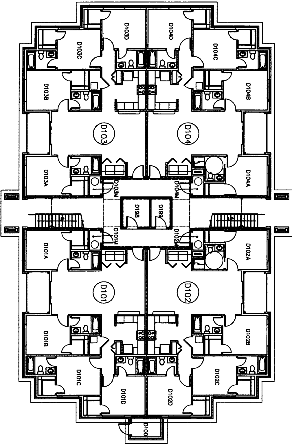
Building "D" - First Floor Plan NOT TO SCALE
